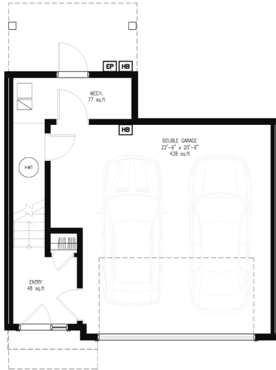
Garage and Lower Floor
